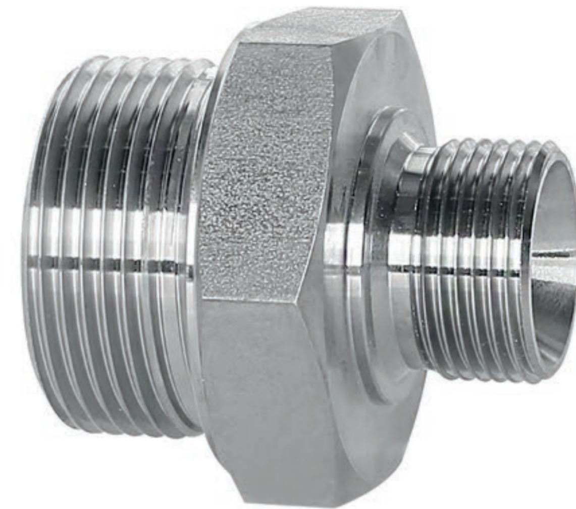
1 1/4" to 3/4" BSP reducing nipple 316 SS quality
