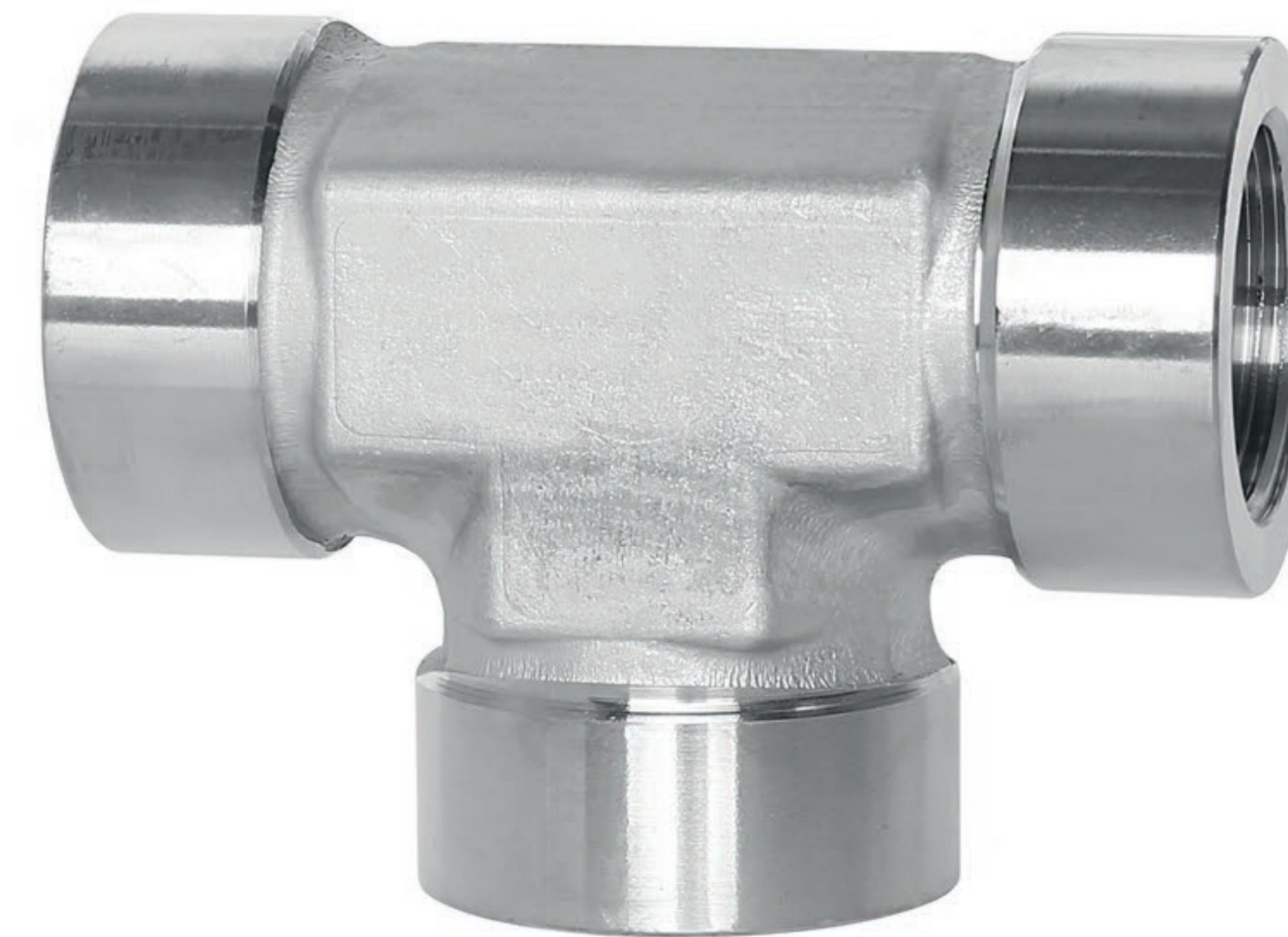
Equal T fitting female 1" thread BSP 303
