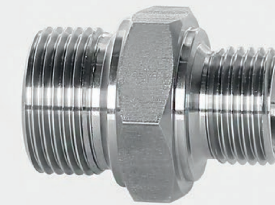
3/4" to 1/2" BSP reducing nipple 316 SS quality
