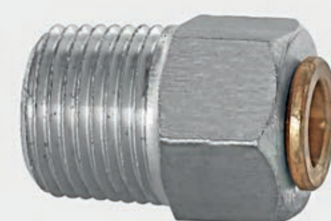
3/8" male connector for 5/16" tube NPT
