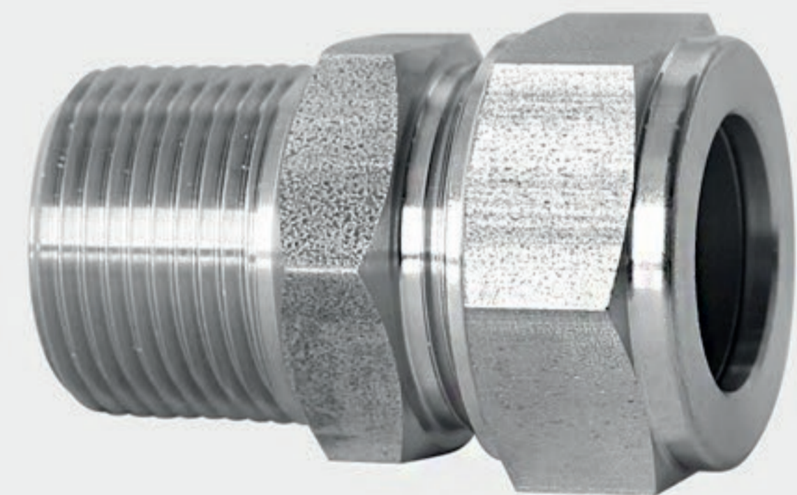
3/4" male NPT connector to 20 SS tube
