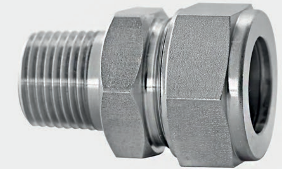
1/2" male NPT connector for 20 tube
