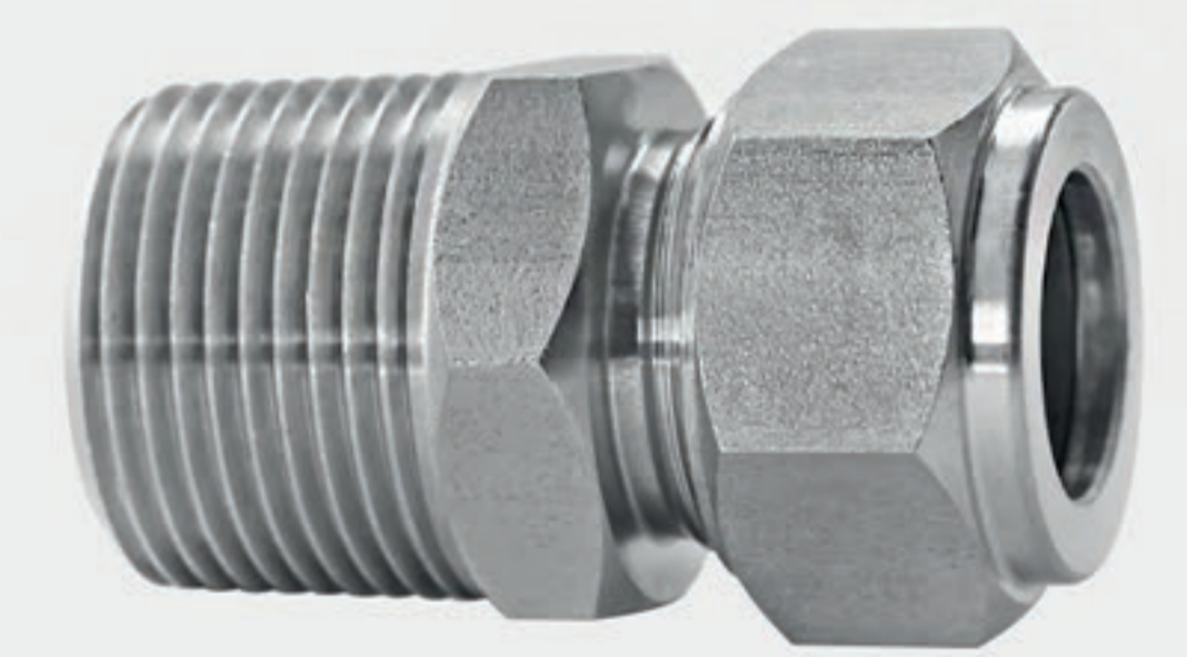
3/4" male NPT connector for 16 mm tube 303
