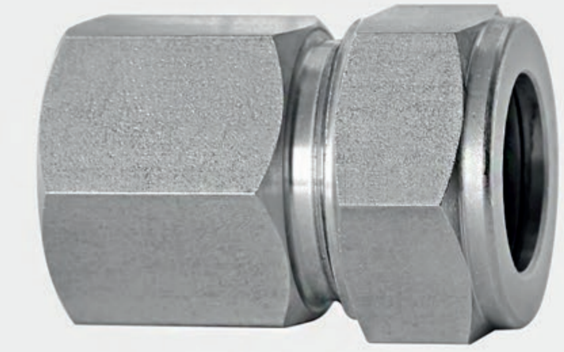
1/2" female NPT connector for 20 tube
