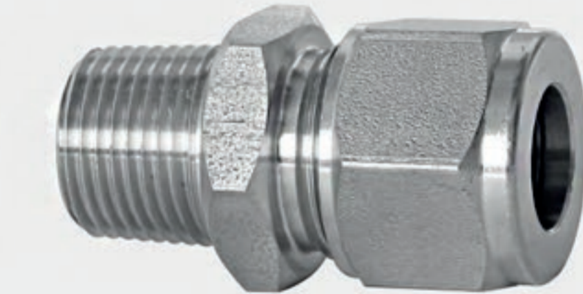
3/8" male NPT connector for 1/2" tube 303
